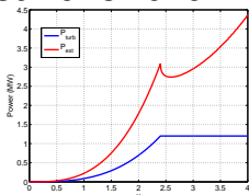
Power Curve vs Power Extraction:
